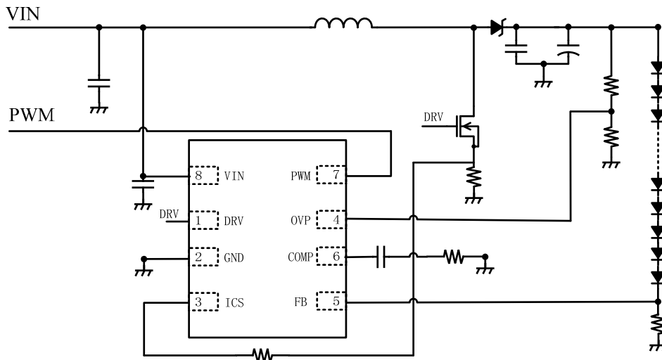
Fig 1 EUP2950C PWM Dimming for White LED Application
